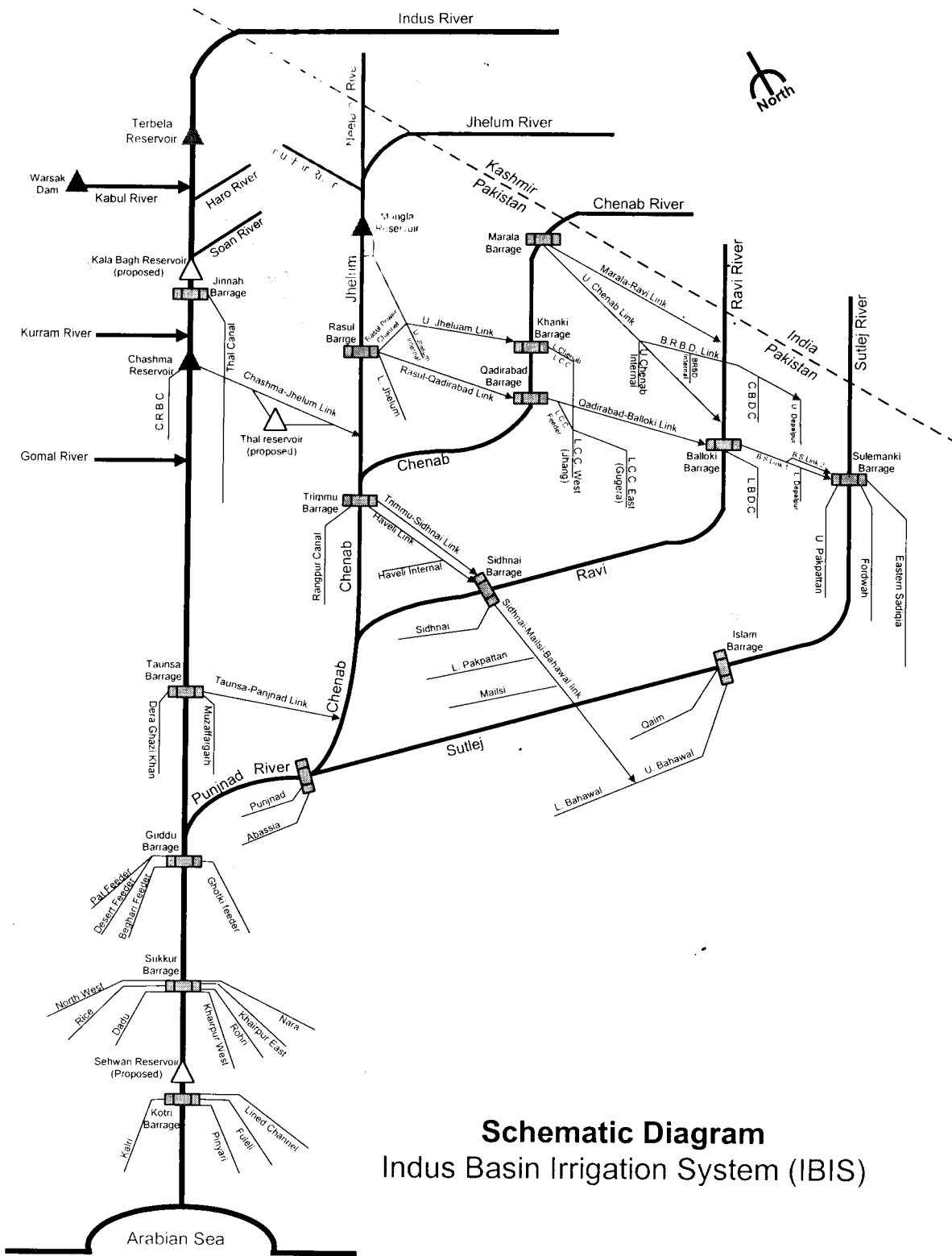
Figure 1.2. The Indus Basin Irrigation System (IBIS), Schematic Diagram.
