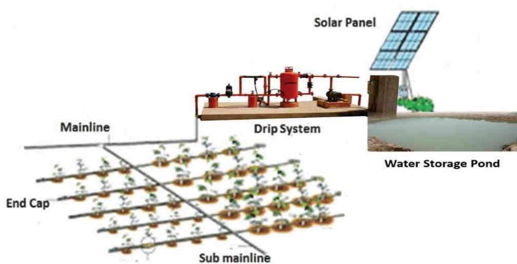
Figure-3: Typical Layout of Solar Powered Drip System (Storage Pond)
