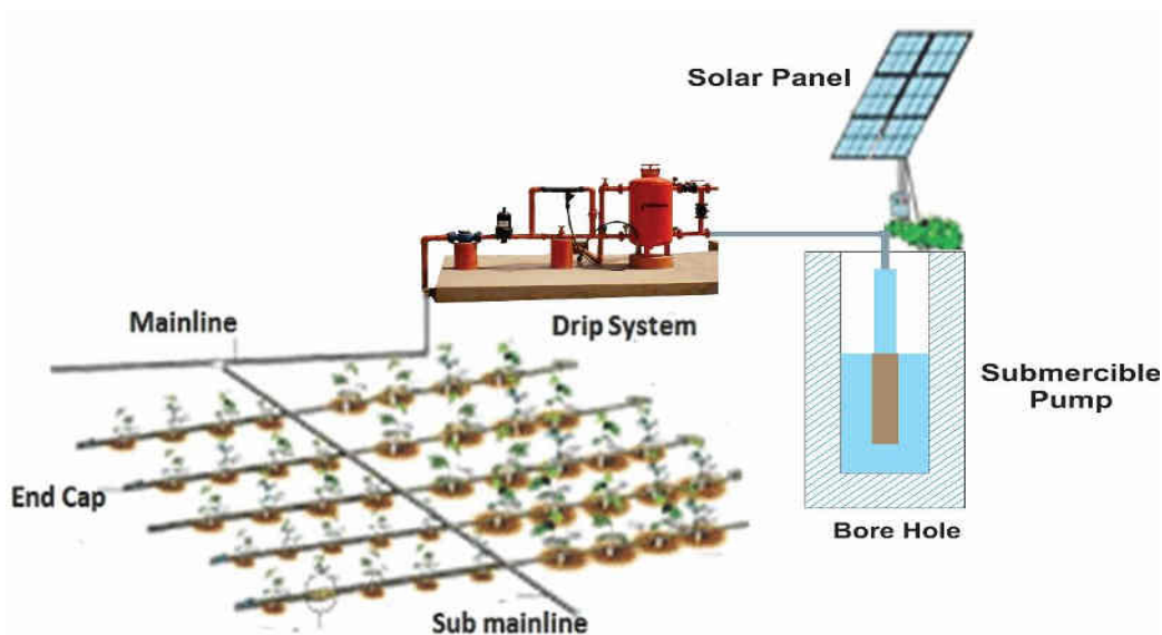
Figure-4: Typical Layout of Solar Powered Drip System (Direct Groundwater Pumping)
