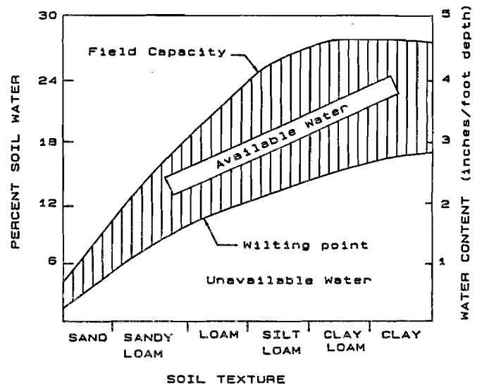
Figure 3. Soil texture as it affects “average” available water capacity
